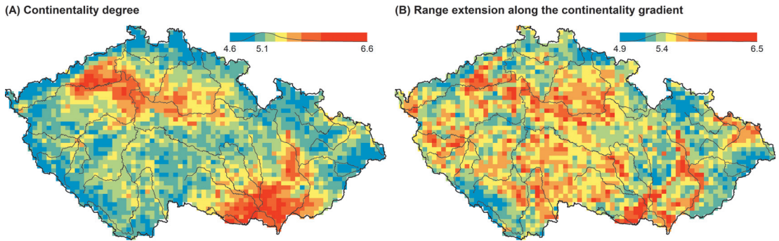
Fig. 32. – Mean continentality degree and mean range extension along the continentality gradient (number of adjacent regions) of species of the Czech flora. The highest mean degree of continentality is found in dry and warm forest-steppe regions of northern and central Bohemia and southern Moravia. The highest range extension along the continentality gradient is encountered in the flora along lowland rivers.
