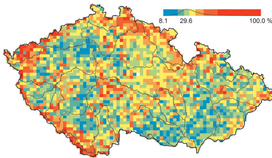
Fig. 27. – Proportion of the deliberately introduced alien species in the Czech alien flora (native species are not considered). Deliberately introduced aliens are particularly frequent in the mountain areas of the Bohemian Massif, whereas accidentally introduced aliens prevail in the lowlands. Note that the absolute number of alien species in the mountain areas is low.
