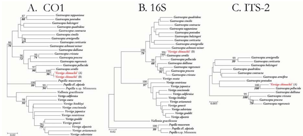
FIGURE 2. Phylogram showing the distribution of analyzed Gastrocopta , Vertigo , Vallonia and Pupilla species based on A. COI ; B. 16S ; and C. ITS-2 . Nodes with support values of approximately 70 or more across both NNJ and ML have been labeled by two numbers to the left of each node. The upper (normal font) represents the NNJ support values while the lower ( bold italic font ) represents ML values. Bottom scale bar is presented in Maximum Composite Distance.
