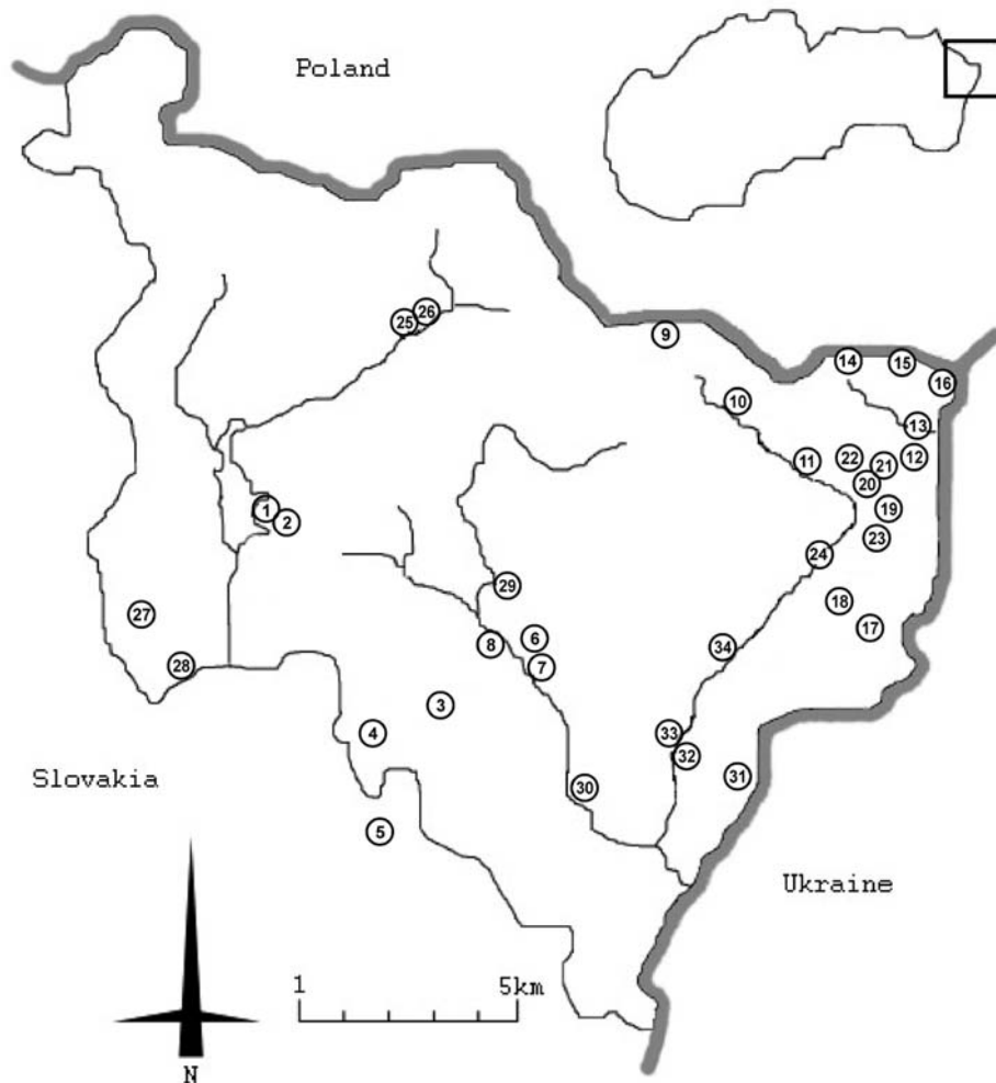
Fig. 1. Location of the study area with positions of the collecting sites (numbers in circles correspond to the list of localities).
