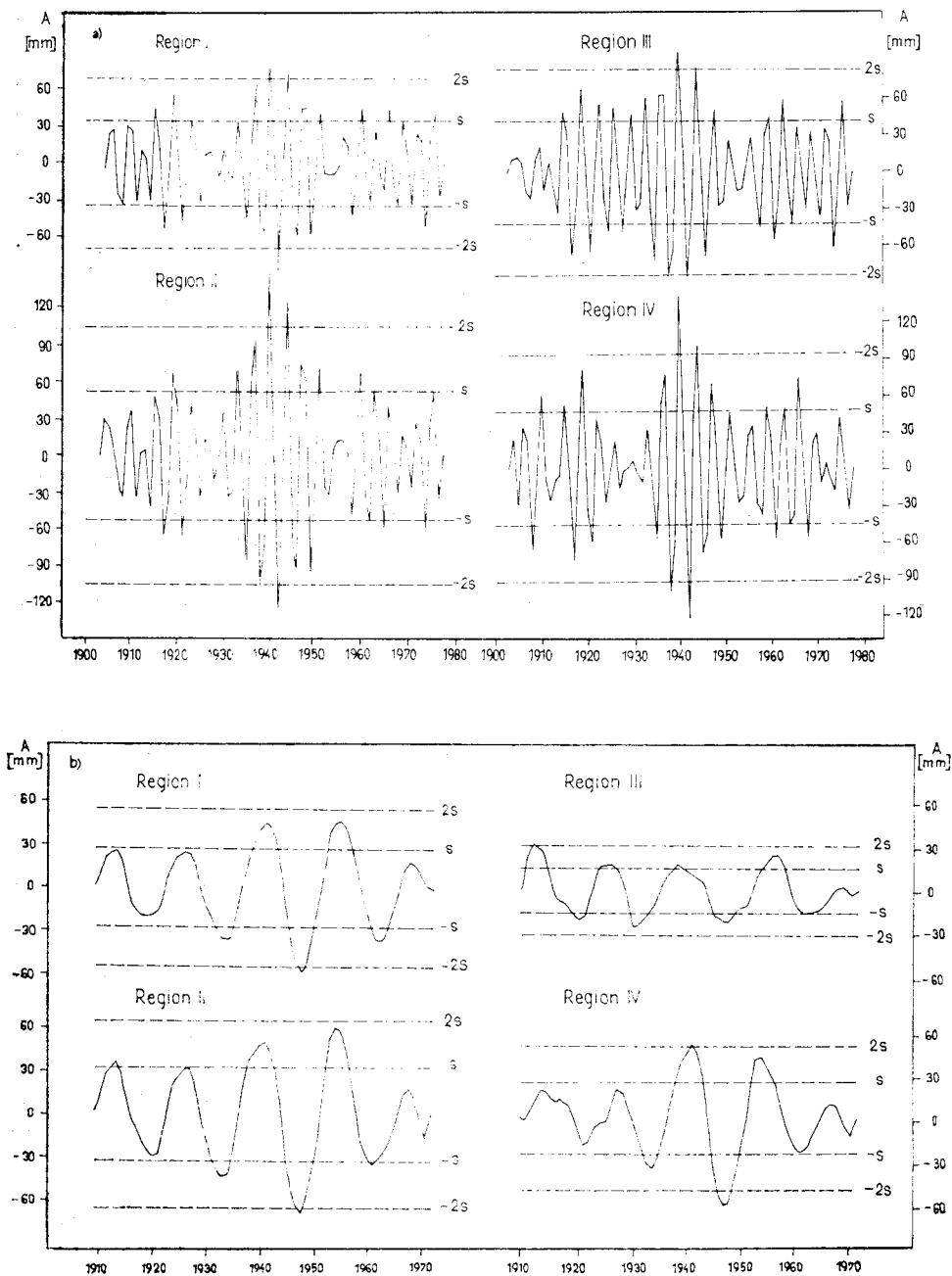
Fig. 6. Numerical band-pass filtering of series of areal annual precipitation sums for different regions of Bulgaria for cycles T = 4a (a) and T = 15a (b). Explanation: s — standard deviation, A — amplitude
